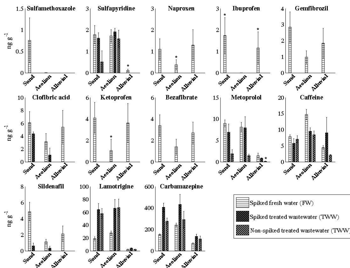
Figure 1. Concentrations of pharmaceuticals in leaves of cucumber plants (ng g -1 dry weight) grown in sandy soil (Sand), aeolian soil (Aeolian), or alluvial soil (Alluvial) and irrigated with spiked fresh water (FW) or spiked or nonspiked treated wastewater (TWW). Mean values and standard error are presented ( n = 9 for spiked FW, n = 4 for spiked and nonspiked TWW). Bars marked with * indicate concentrations between LOD and LOQ.
