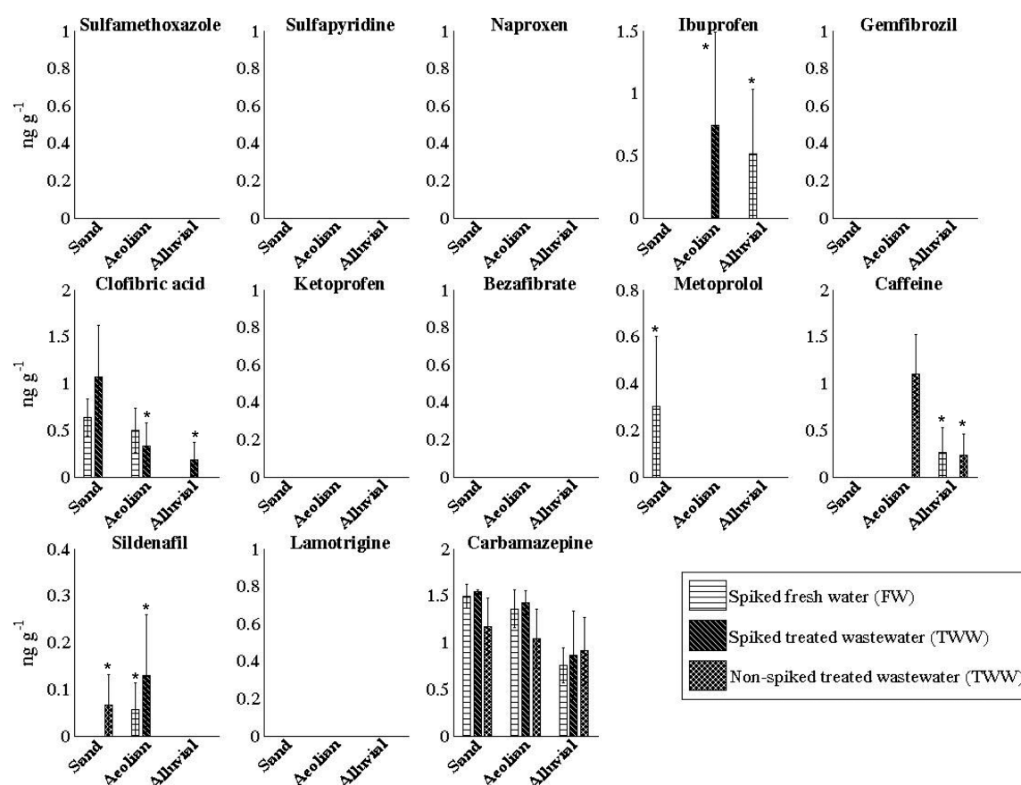
Figure 4. Concentrations of pharmaceuticals in fruit of tomato plants (ng g -1 dry weight) grown in sandy soil (Sand), aeolian soil (Aeolian), or alluvial soil (Alluvial) and irrigated with spiked fresh water (FW), or spiked or nonspiked treated wastewater (TWW). Mean values and standard error are presented ( n = 9 for spiked FW, n = 4 for spiked and nonspiked TWW). Bars marked with * indicate concentrations between LOD and LOQ.
